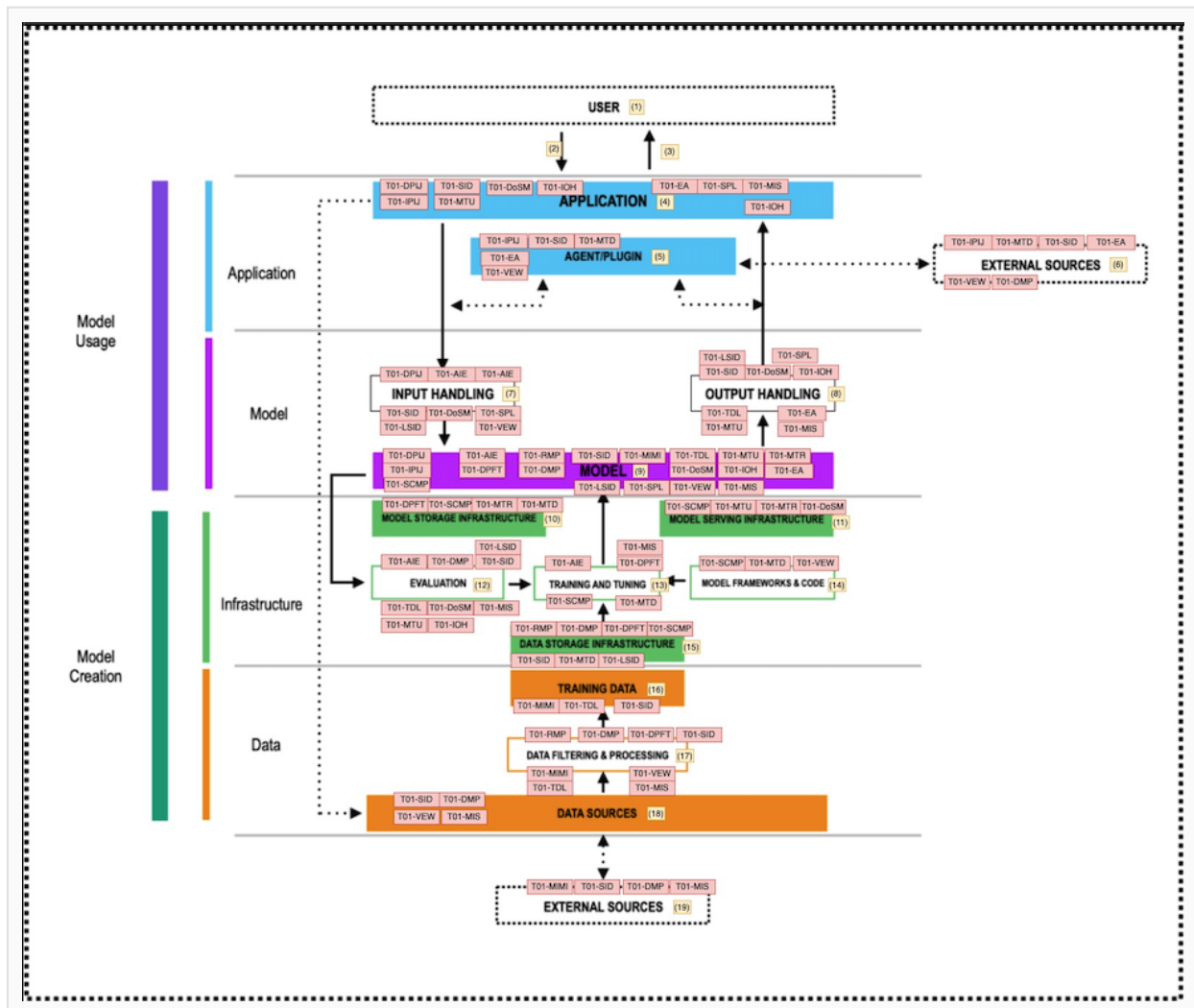
Fig 2.1 Threat Model of OWASP Threats (LLM T10 and AI Exchange) Mapped to Impacted AI Components of a SAIF baseline architecture
