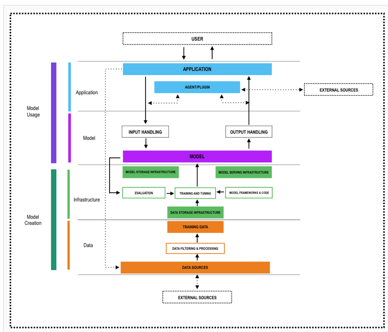
Fig 1.1 SAIF Architecture Layers & Components
